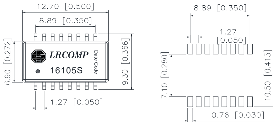
SUGGESTED PCB LAYOUT
