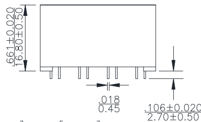
Dimension:mm[Inch]±0.25[0,010]
